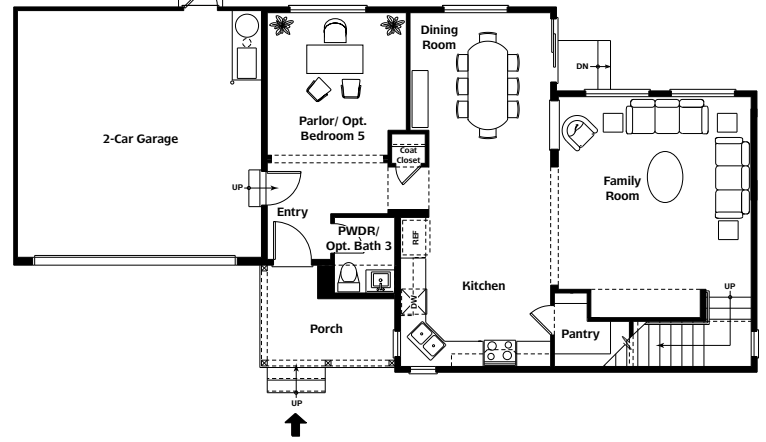
Cottonwood II (1187-2) Main Floor Plan
